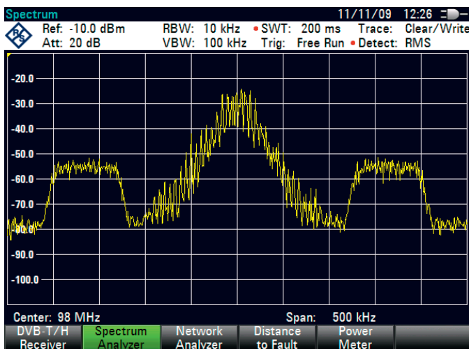
Signal generation for HD Radio™ with the R&S®SFE100-K35 ARB waveform generator.
