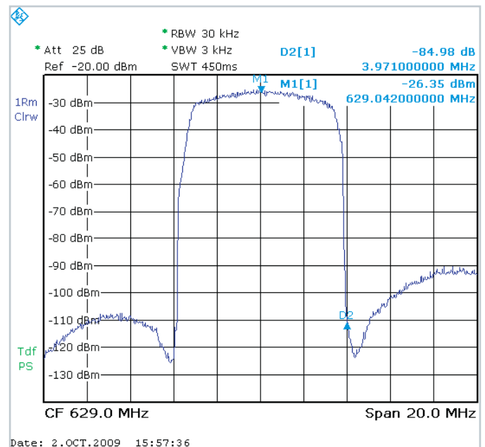
Frequency spectrum with transducer function.
