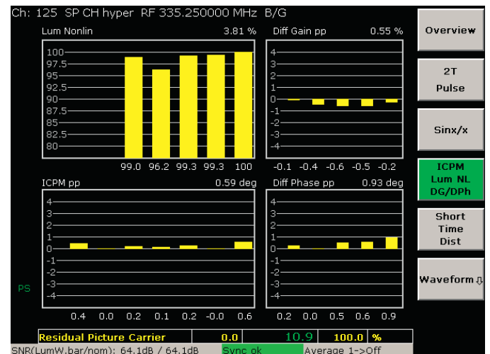
ICPM measurement.
