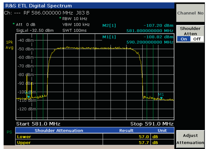
Frequency spectrum of a J.83/B-signal with interferer.
