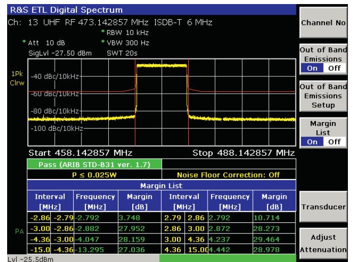
Checking spurious emissions with spectrum mask.
