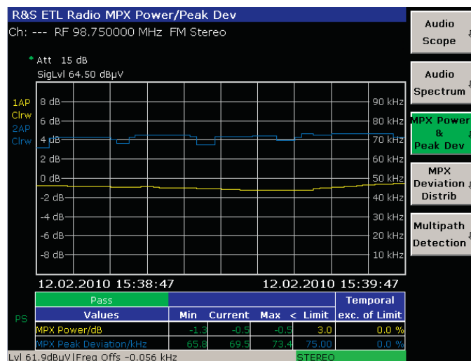
MPX power and peak deviation over 60 s.
