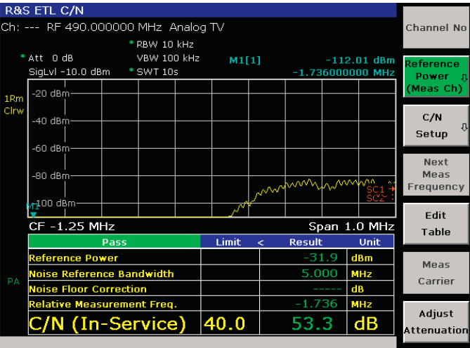
Carrier to noise (C/N) measurement.
