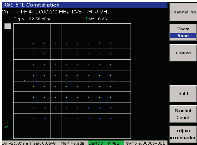
Constellation diagram of a DVB-T, DVB-H signal.
