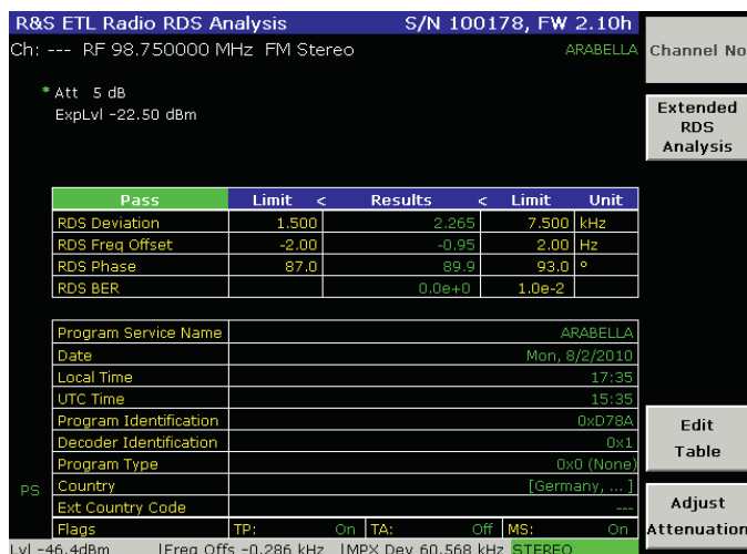
RDS basic information.
