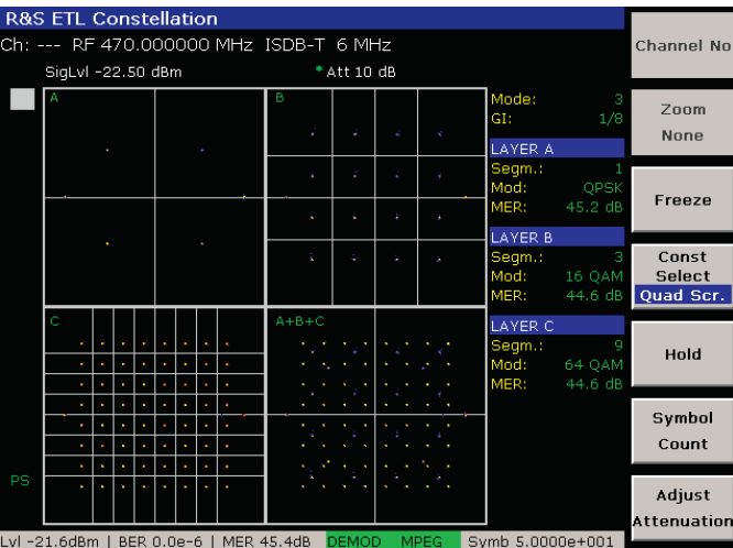
Constellation diagram of an ISDB-T signal.
