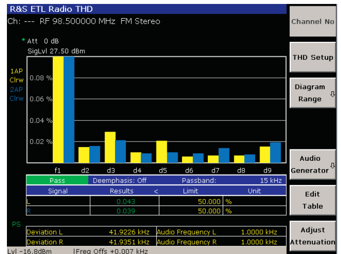
Total harmonic distortion (THD) measurement.
