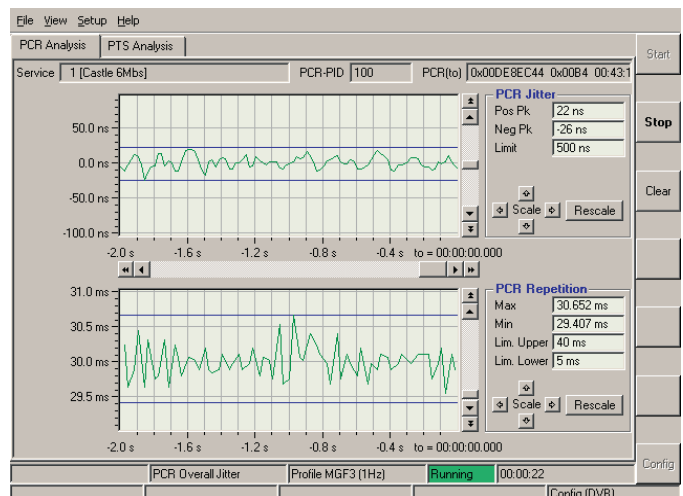
Tracking down PCR jitter.
