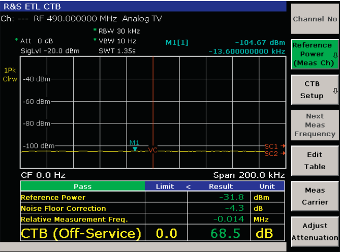
Composite triple beat (CTB) measurement.
