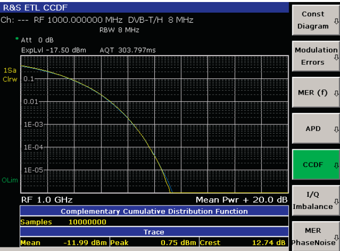
Complementary cumulative distribution function (CCDF) measurement.
