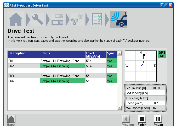
Status messages at a glance during a drive test.
