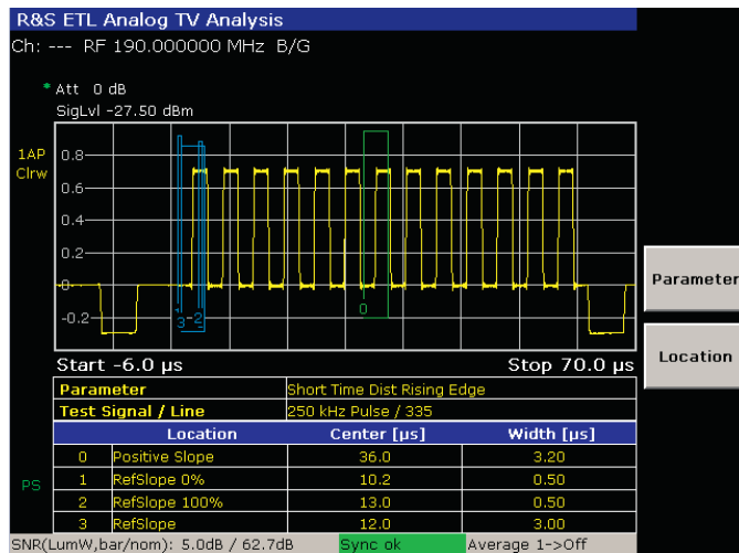
Video test line with measurement parameters.
