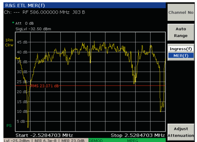
MER (f) of a J.83/B-signal with superimposed interfering.
