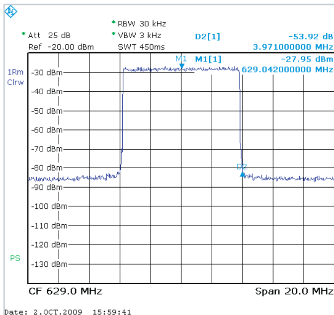
Frequency spectrum without transducer function.
