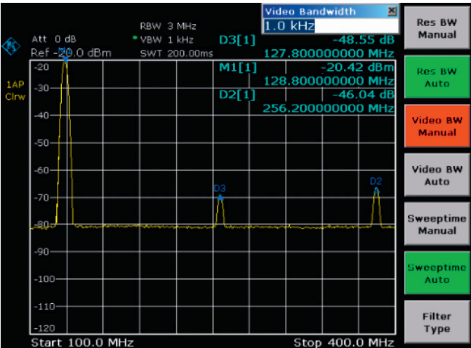
Harmonics measurement.
