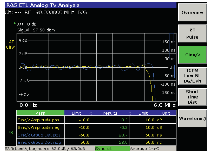
Amplitude and group delay measurement.
