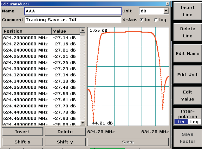
Transducer editor.
