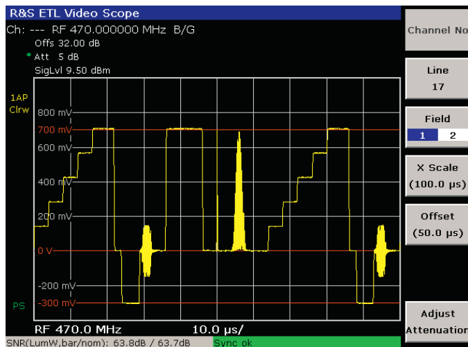
Video line oscilloscope.
