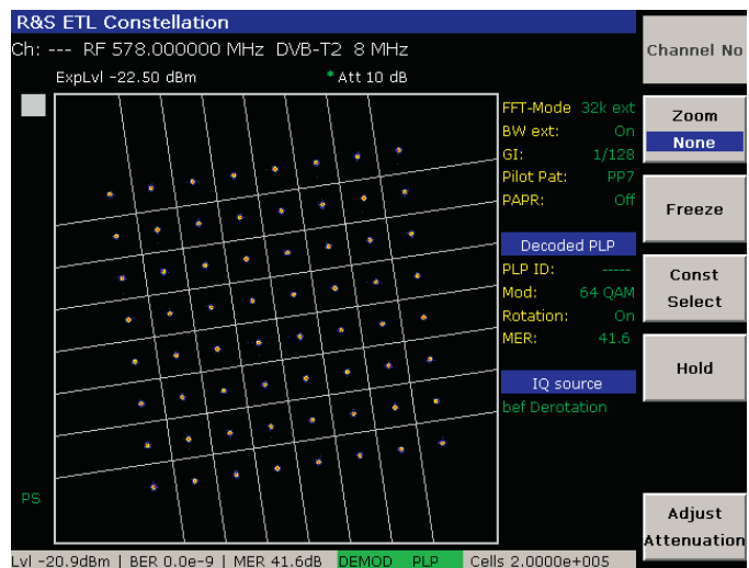
Constellation diagram of a DVB-T2 signal.
