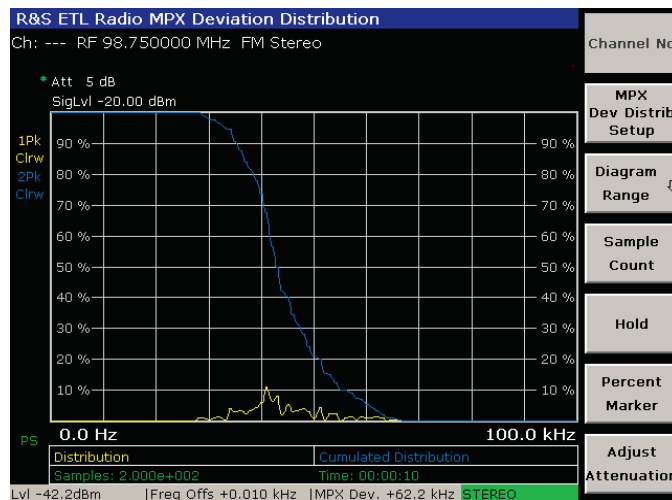
MPX deviation and MPX deviation distribution.
