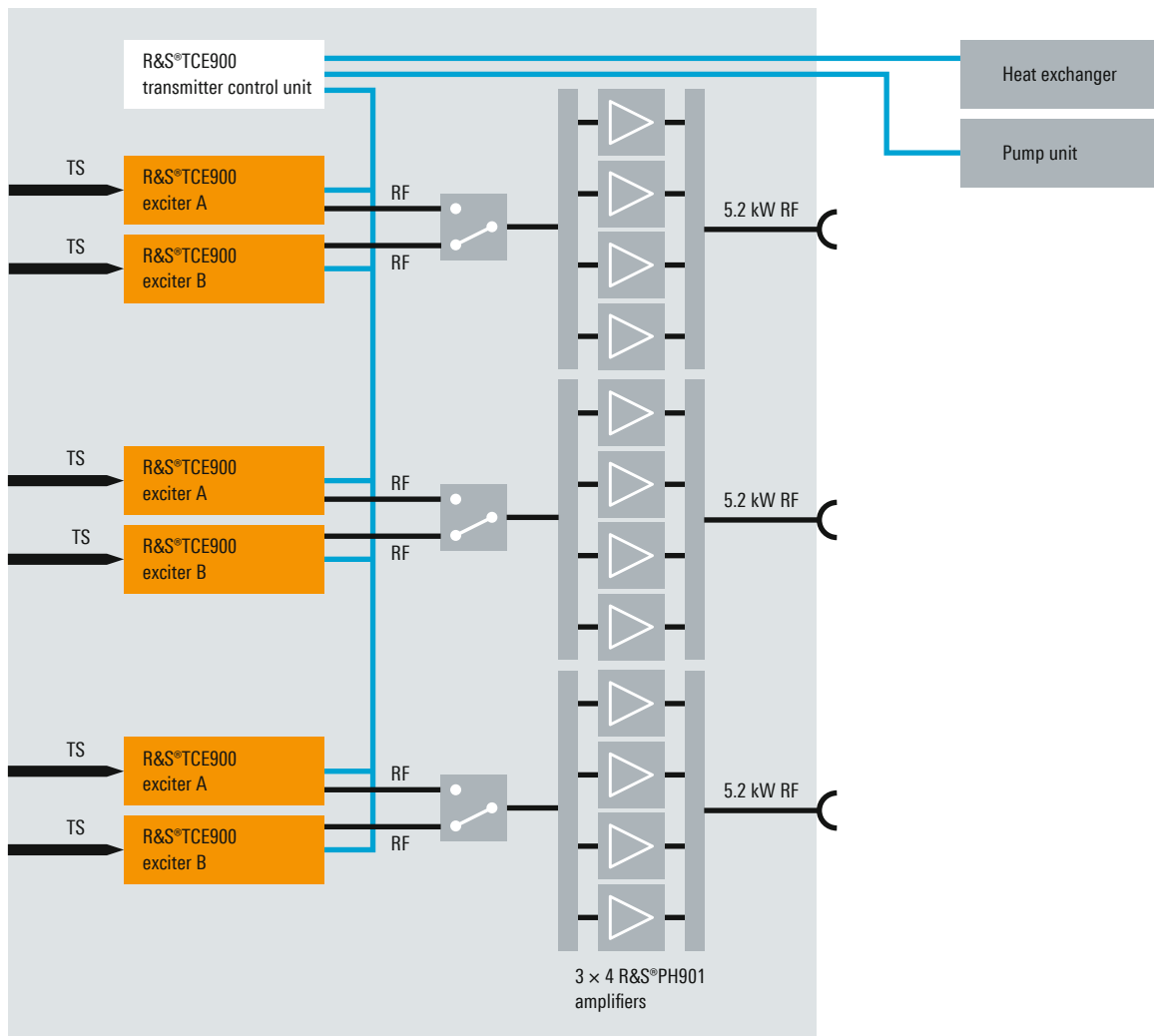
Example of a MultiTX system with three 5.2 kW DVB-T transmitters in a single rack
